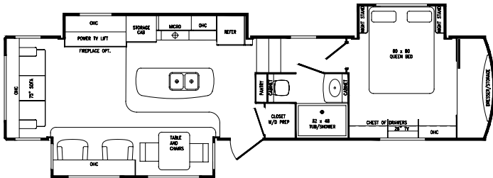
385RSS Length 38' 3" Dry Weight 11,850# • Dry Pin Weight 2,875#
