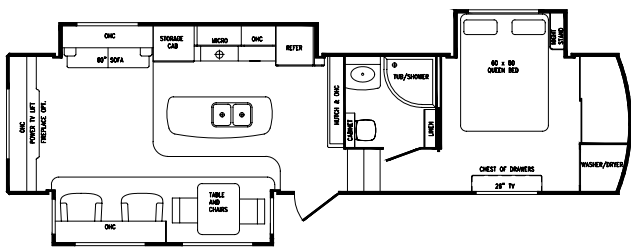
340RES Length 36' 1" Dry Weight 11,725# • Dry Pin Weight 2,950#
