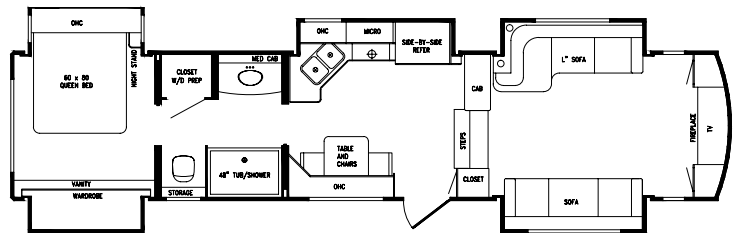
390FLS Length 39' 3" Dry Weight 13,125# • Dry Pin Weight 2,825#
