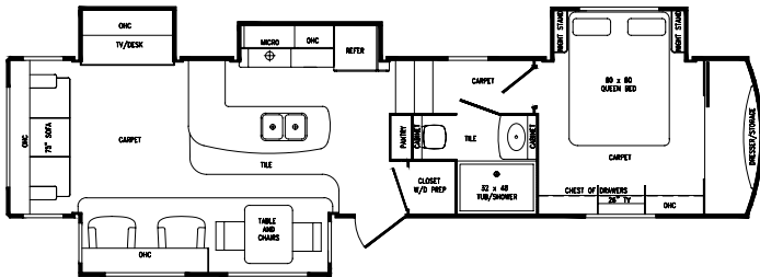
370TKS Length 38' 3" Dry Weight 11,850# • Dry Pin Weight 2,875#
