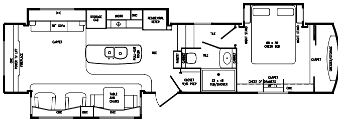
380 RES Length 38' 3" • Dry Weight 12,700# • Dry Pin Weight 2,875#
