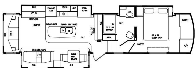
384 RSS Length TBD • Dry Weight 13,250# • Dry Pin Weight TBD
