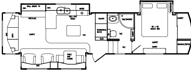
365 LKS Length TBD • Dry Weight 12,700# • Dry Pin Weight TBD
