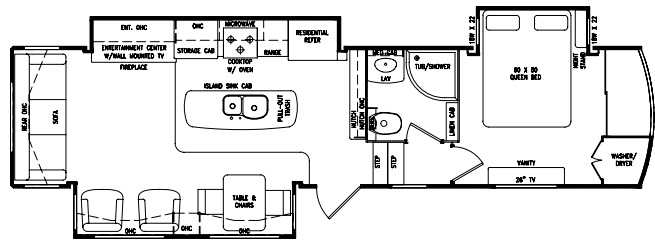
360 RSS Length 37' 1" • Dry Weight 12,500# • Dry Pin Weight 2,875#
