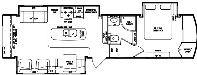
340 RES Length 36' 1" • Dry Weight 11,725# • Dry Pin Weight 2,950#
