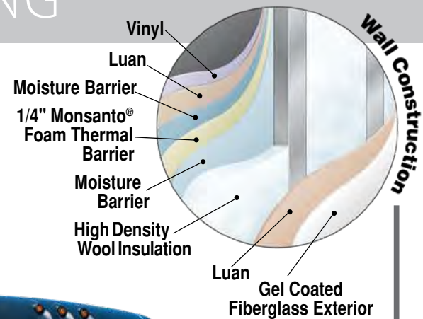
Residential Sidewall R16
