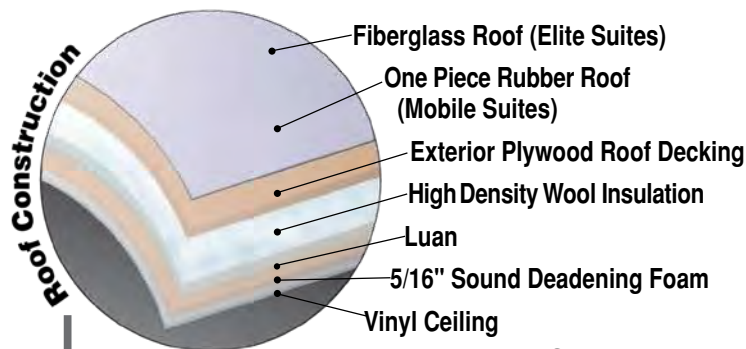
Residential Roof R25
