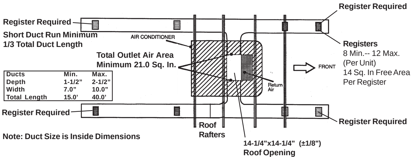
FIG. 7B Duct Size And Requirements For 3308120 Genesis Air Filtration System Kit
