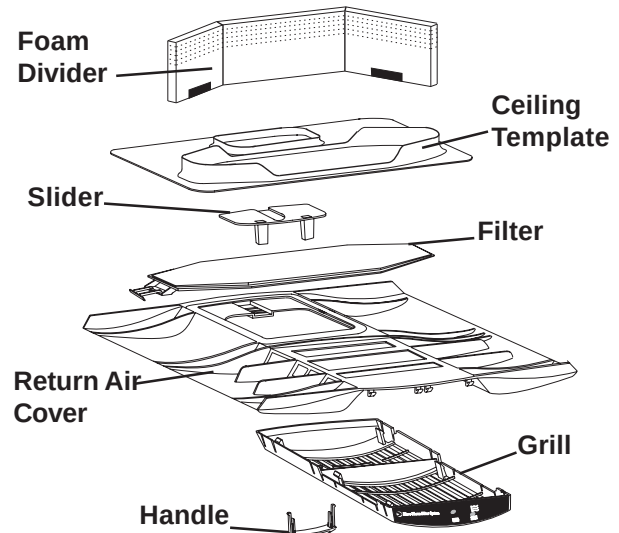
FIG. 25 Genesis Air Filtration System Return Air Kit
