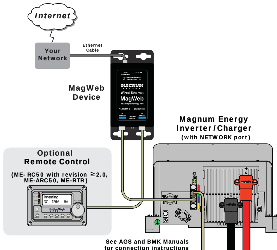
Figure 2-1, MagWeb System Diagram (not to scale)
