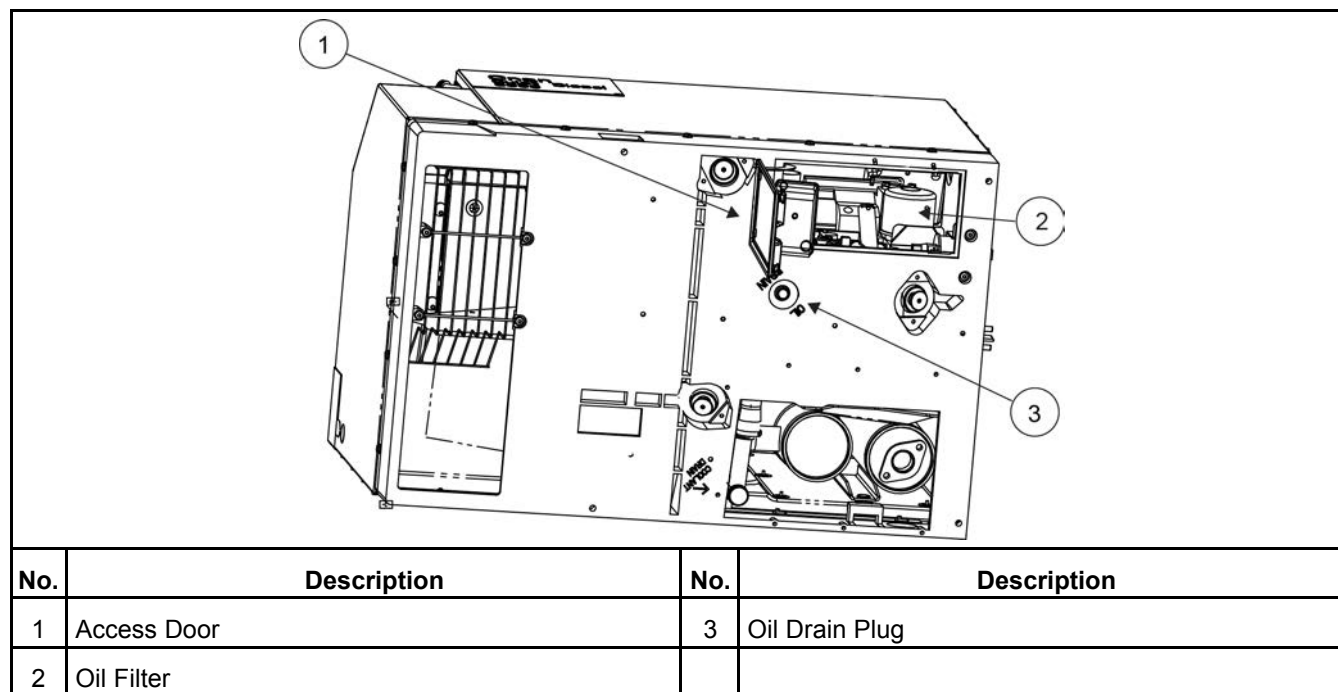
FIGURE 6. OIL DRAIN PLUG(S)
