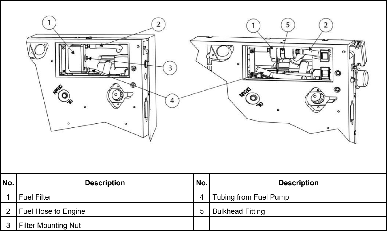
FIGURE 7. FUEL FILTER
