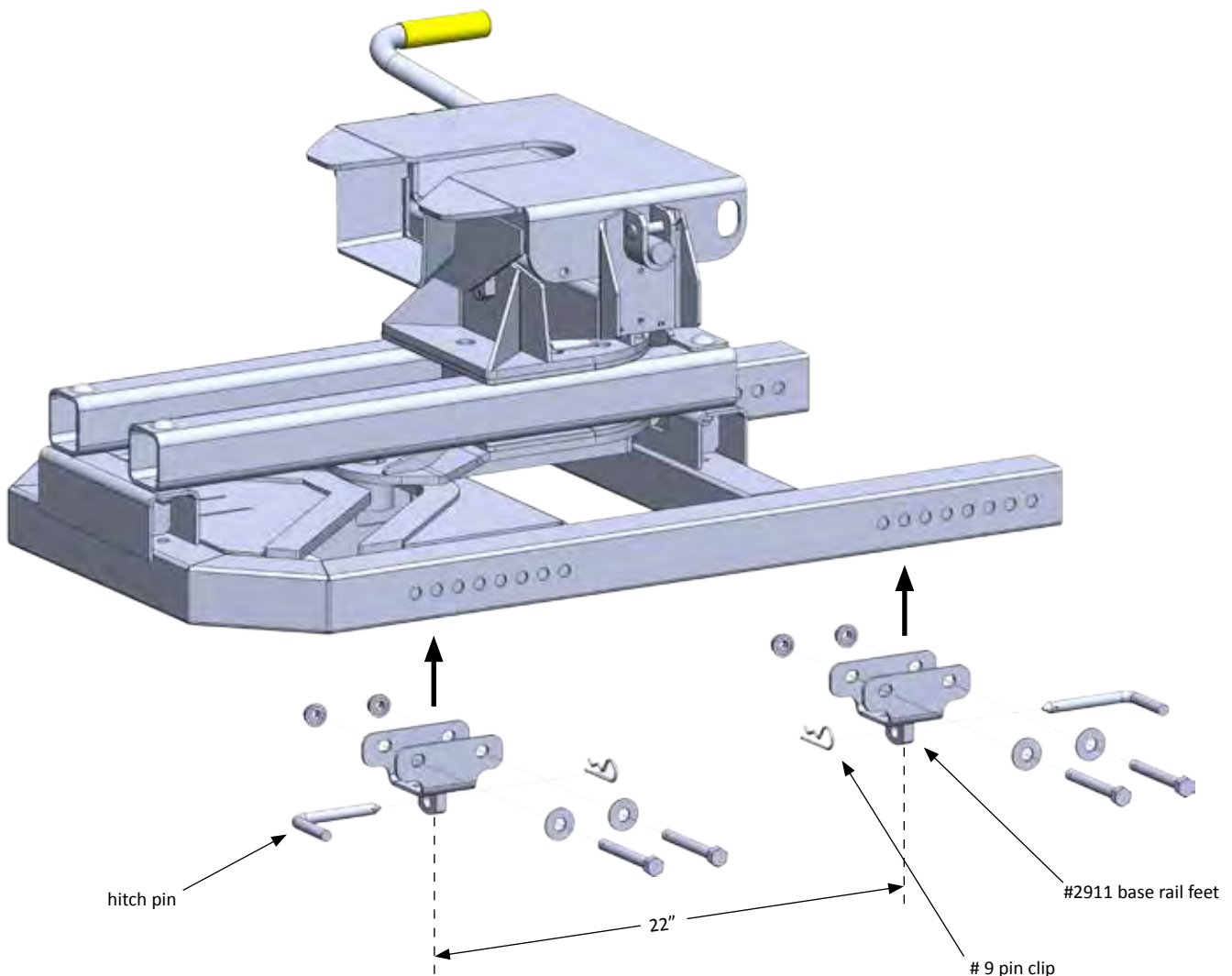
BASE RAIL FOOT ASSEMBLIES — EXPLODED VIEW
